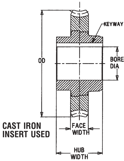
SOLID SHAFT GEAR
