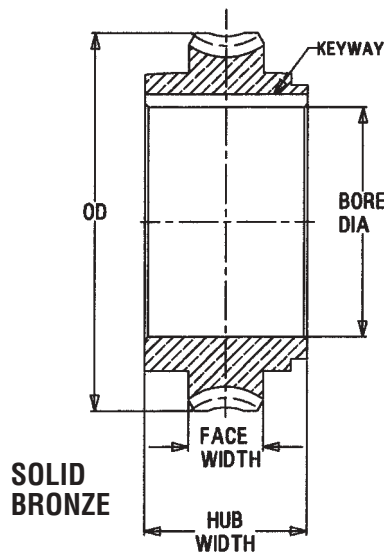
HOLLOW SHAFT GEAR
